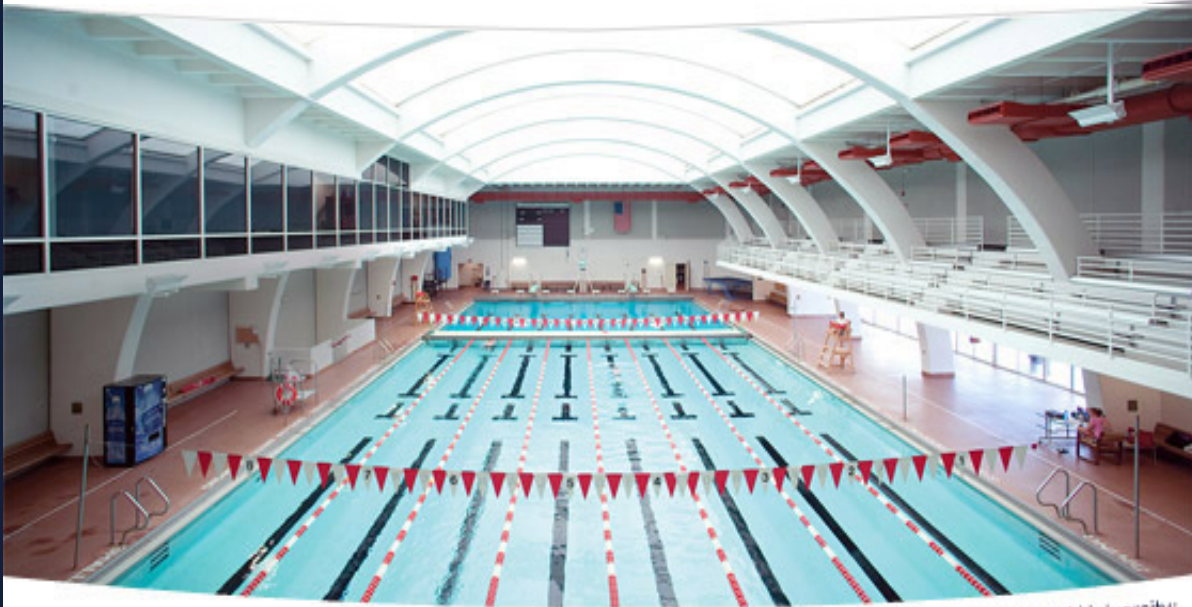
Dedmon Center at Radford University: the world's first insulated translucent membrane roof
